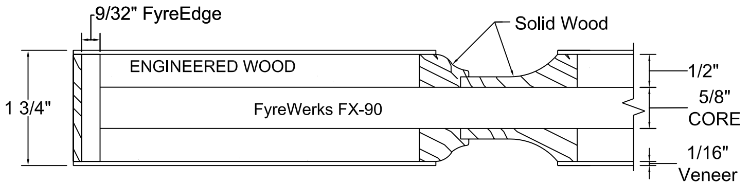
90-Minute Rated - Category "A"
