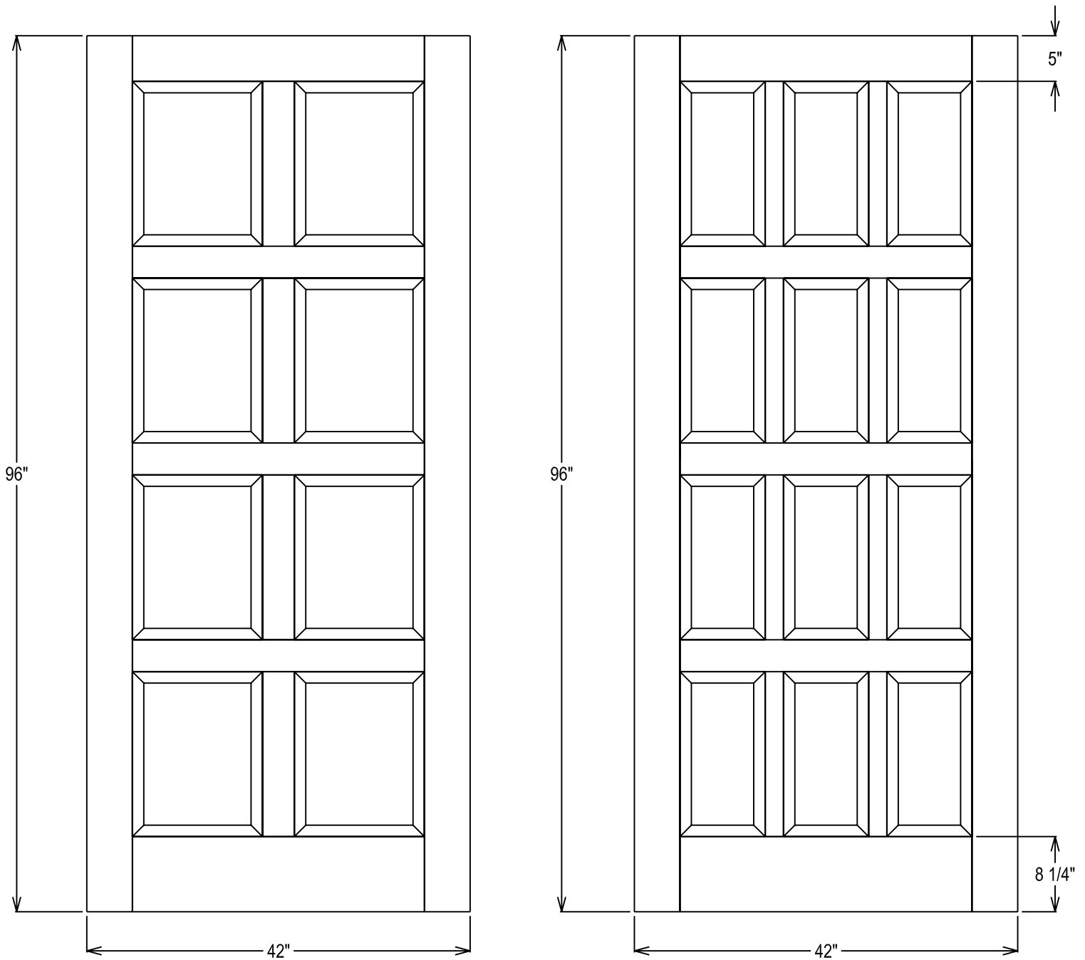
60-Minute Rating, 8&12-Panel Layout
