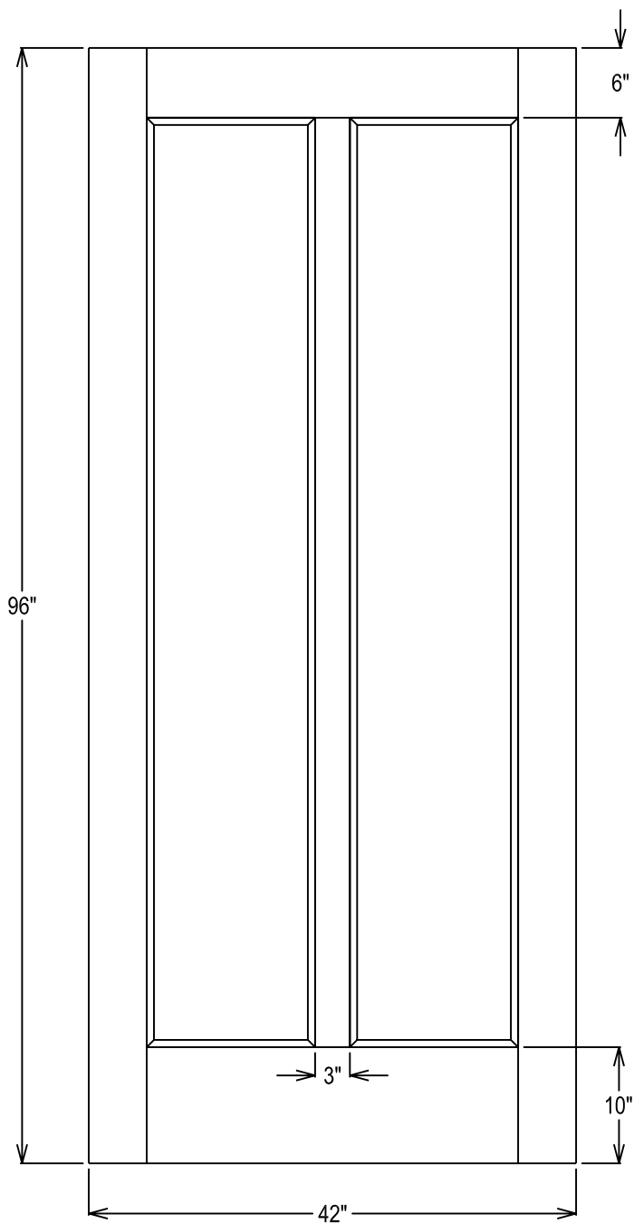
60-Minute Rating, 2-Panel Layout
