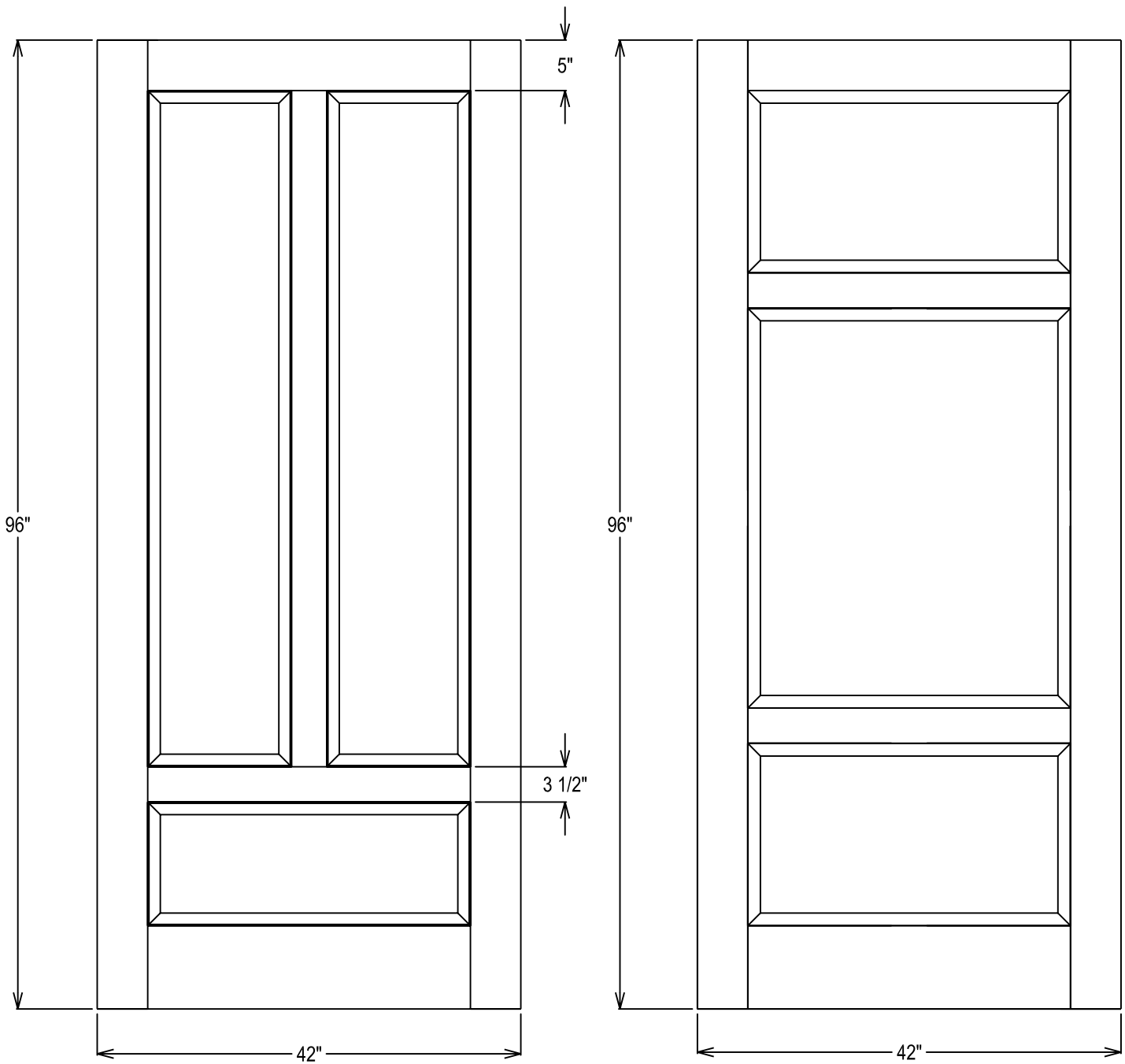
60-Minute Rating, 3-Panel Layout
