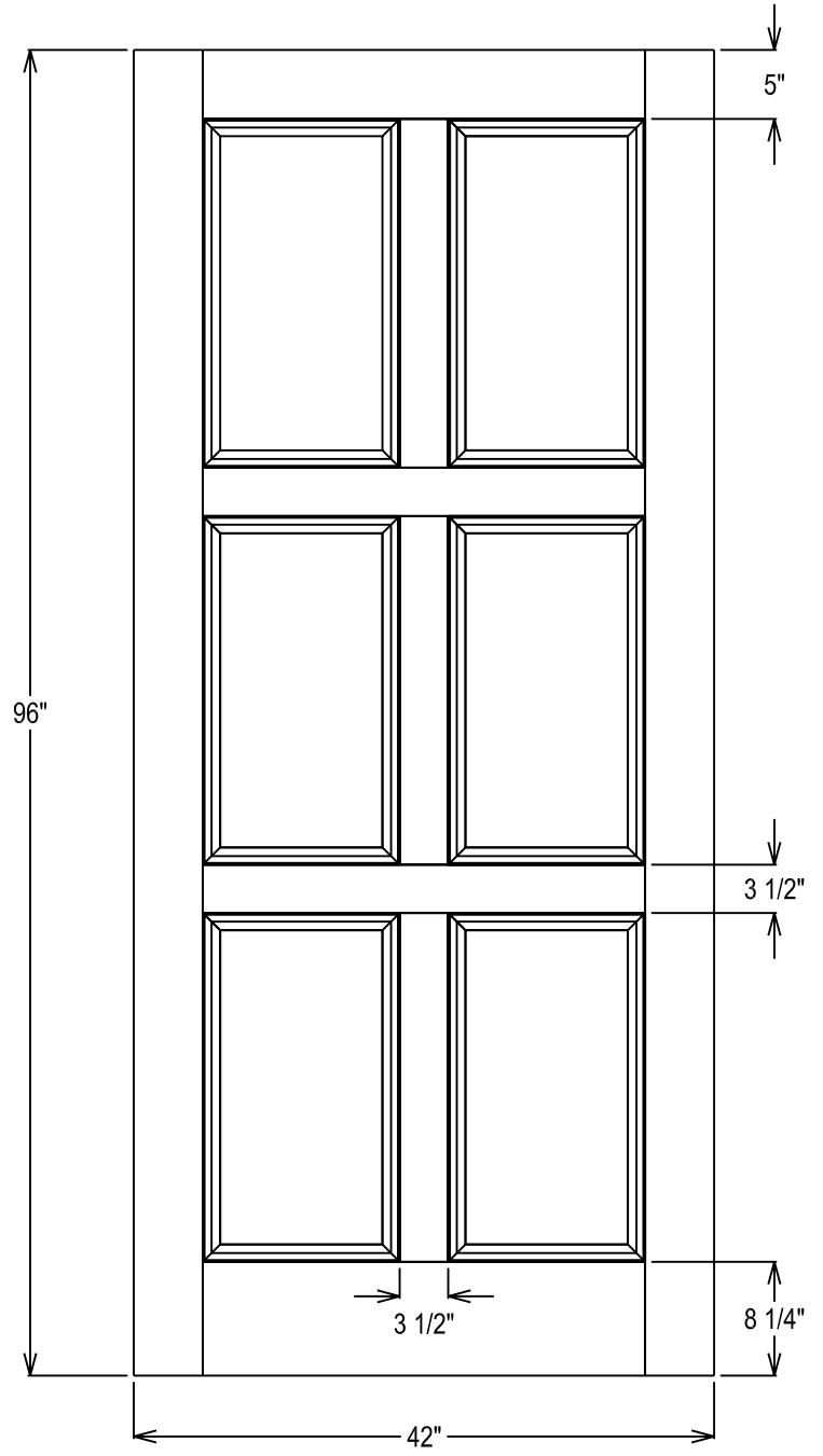
60-Minute Rating, 5&6-Panel Layout
