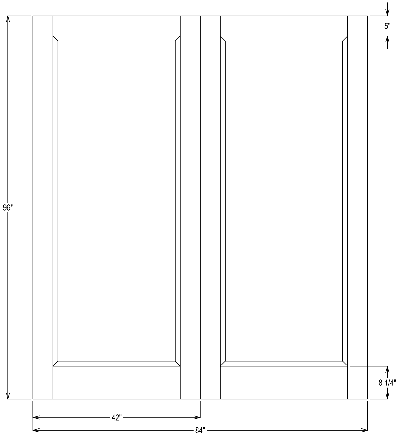
60-Minute Rating, Paired Doors, 1-Panel Layout
