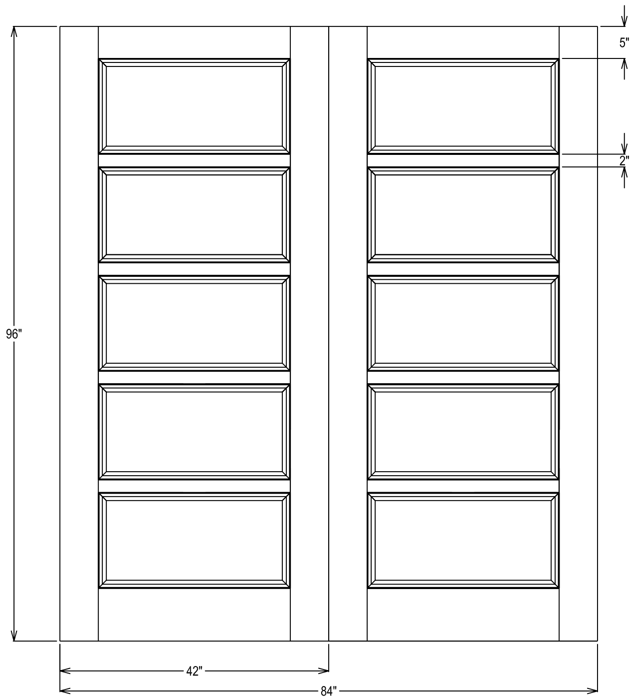
60-Minute Rating, Paired Doors, 5-Panel Layout
