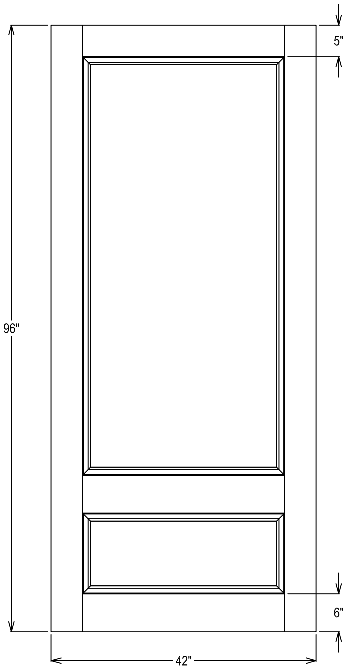
60-Minute Rating, 2-Panel Layout
