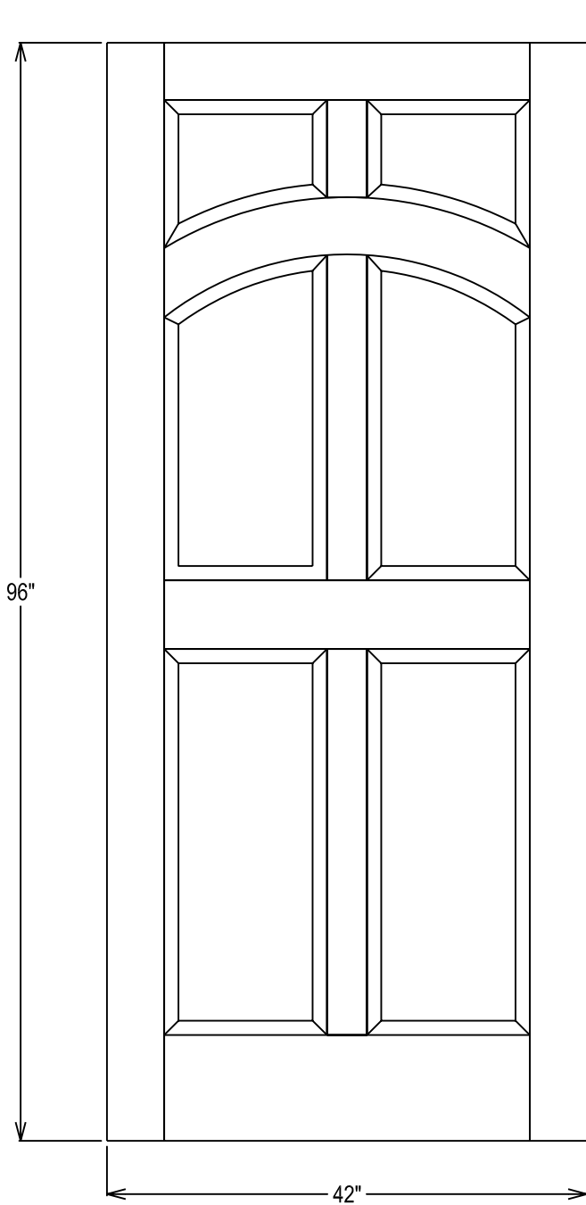
60-Minute Rating, 6-Panel Layout
