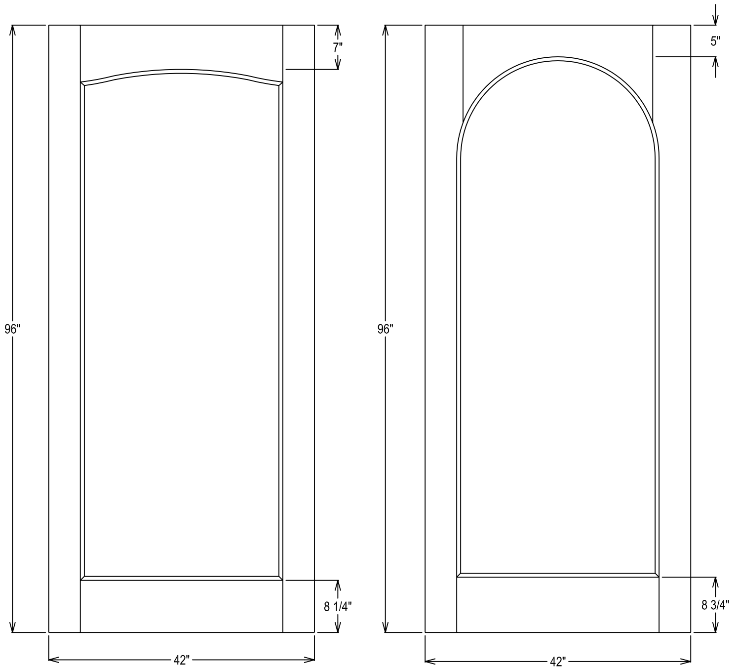
60-Minute Rating, 1-Panel Layout
