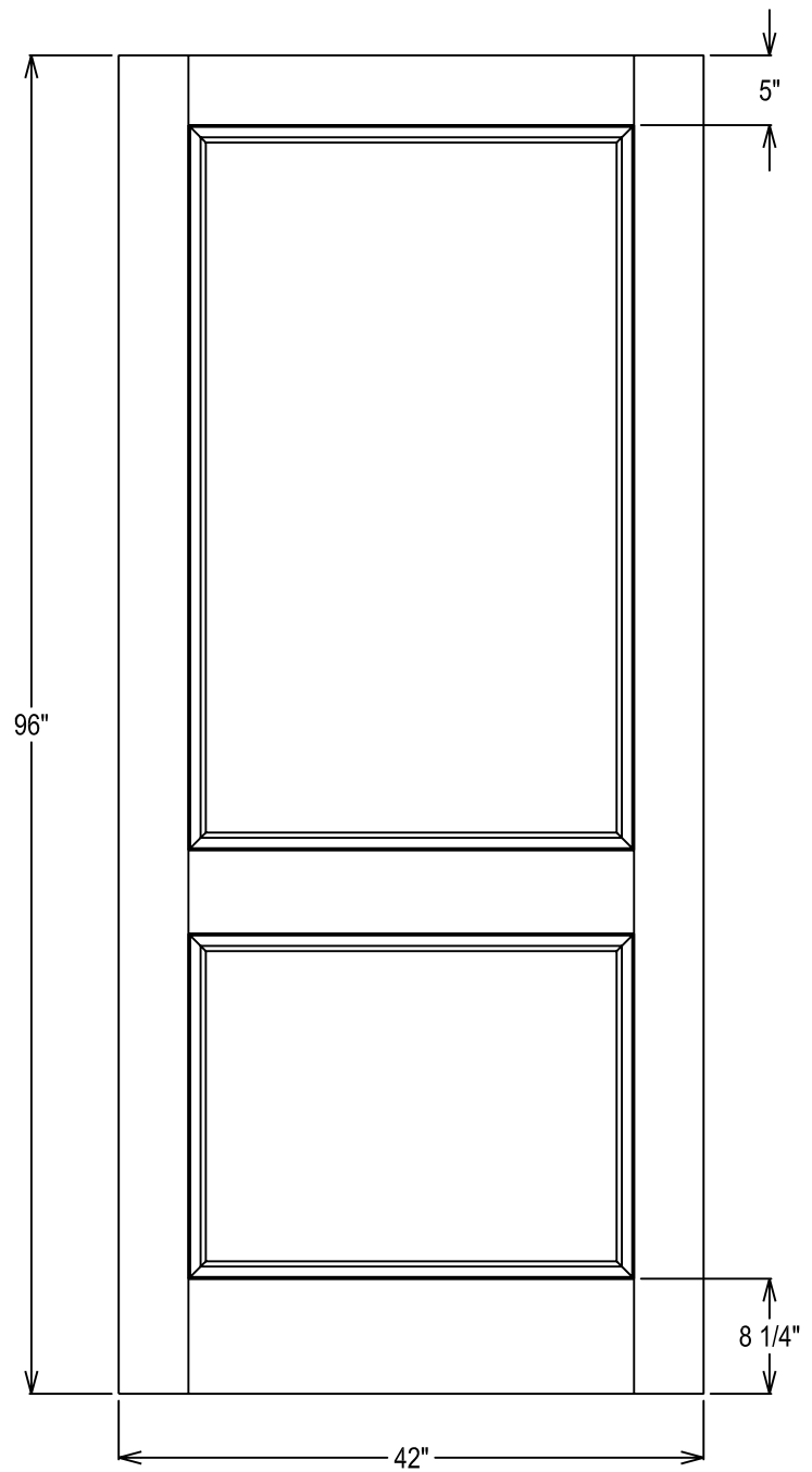
60-Minute Rating, 2-Panel Layout
