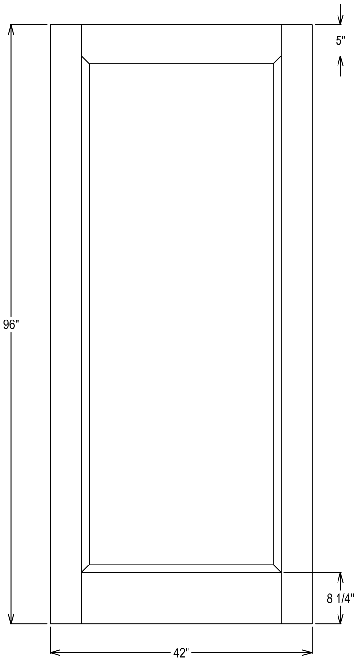
60-Minute Rating, 1-Panel Layout
