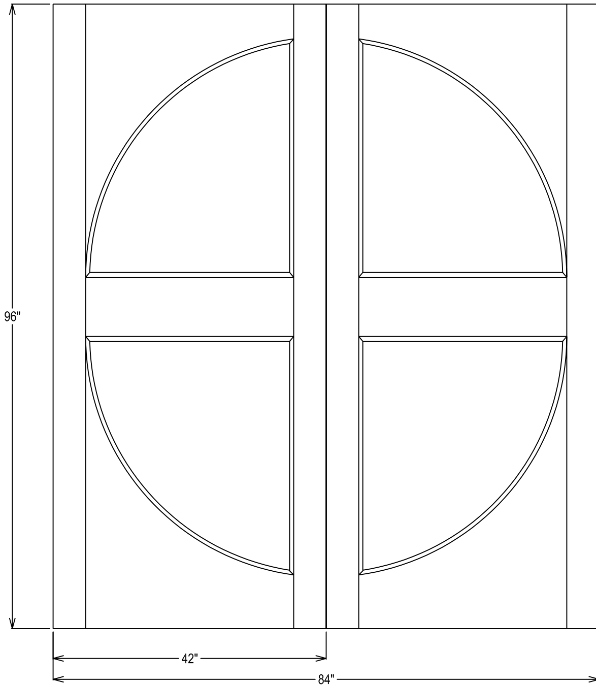
60-Minute Rating, Paired Doors, 2-Panel Layout
