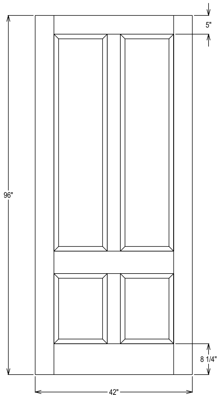
60-Minute Rating, 4-Panel Layout
