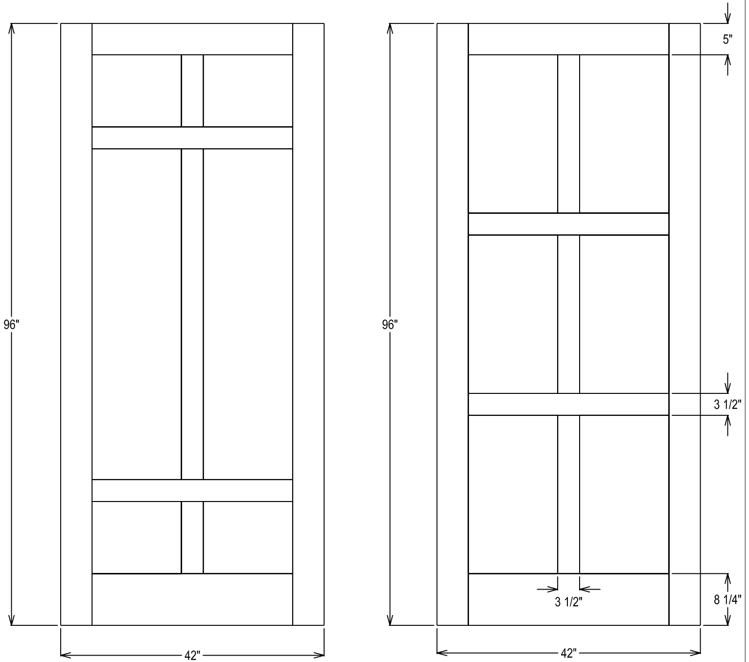
20-Minute Rating, 6-Panel Layout
