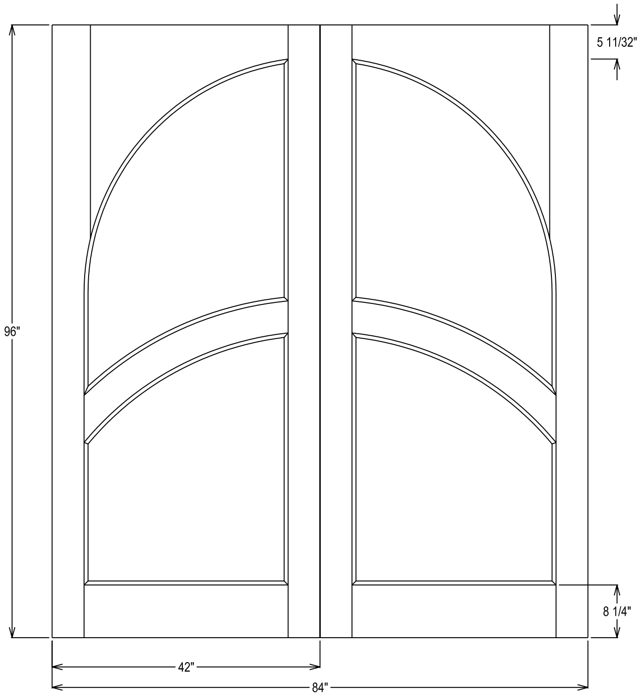
20-Minute Rating, Paired Doors, 2-Panel Layout
