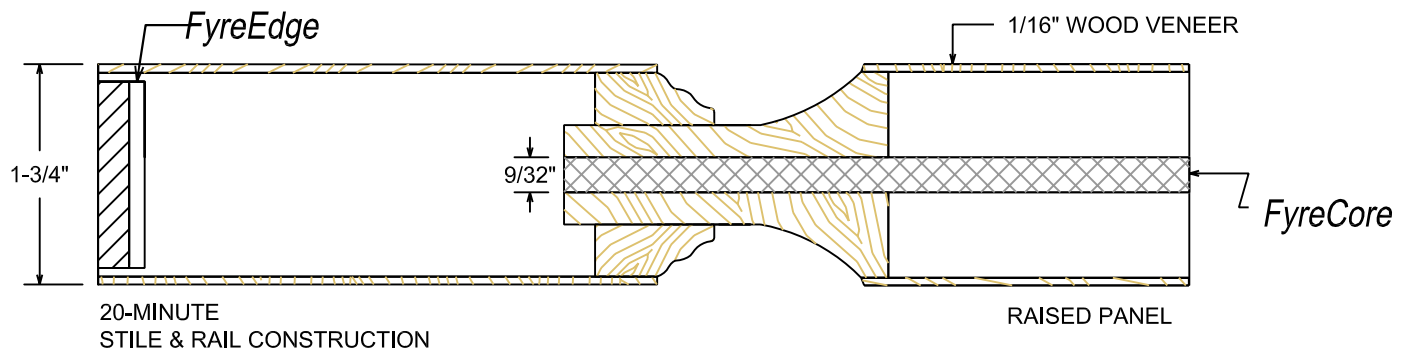
20-Minute Rating, Paired Doors, 5-Panel Layout
