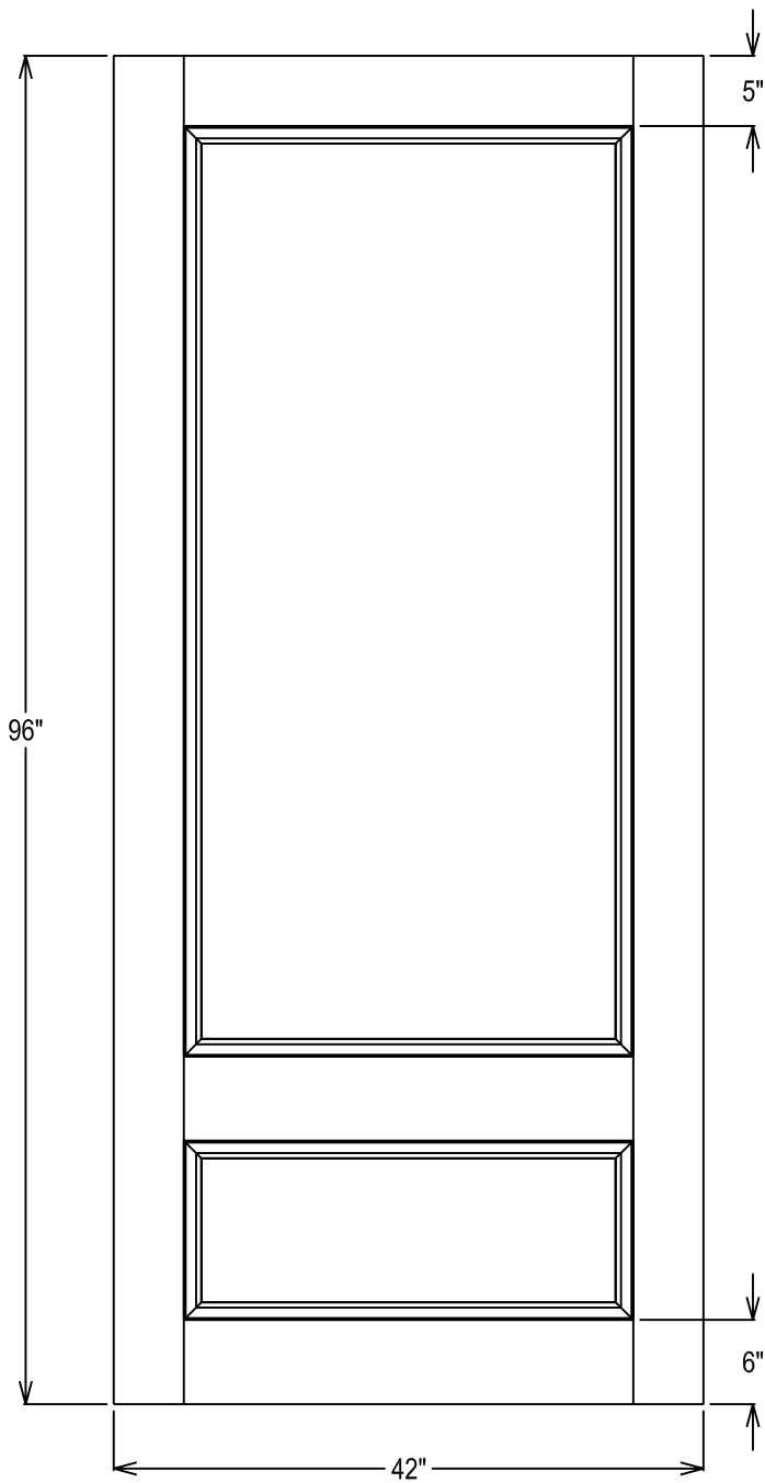
20-Minute Rating, 2-Panel Layout
