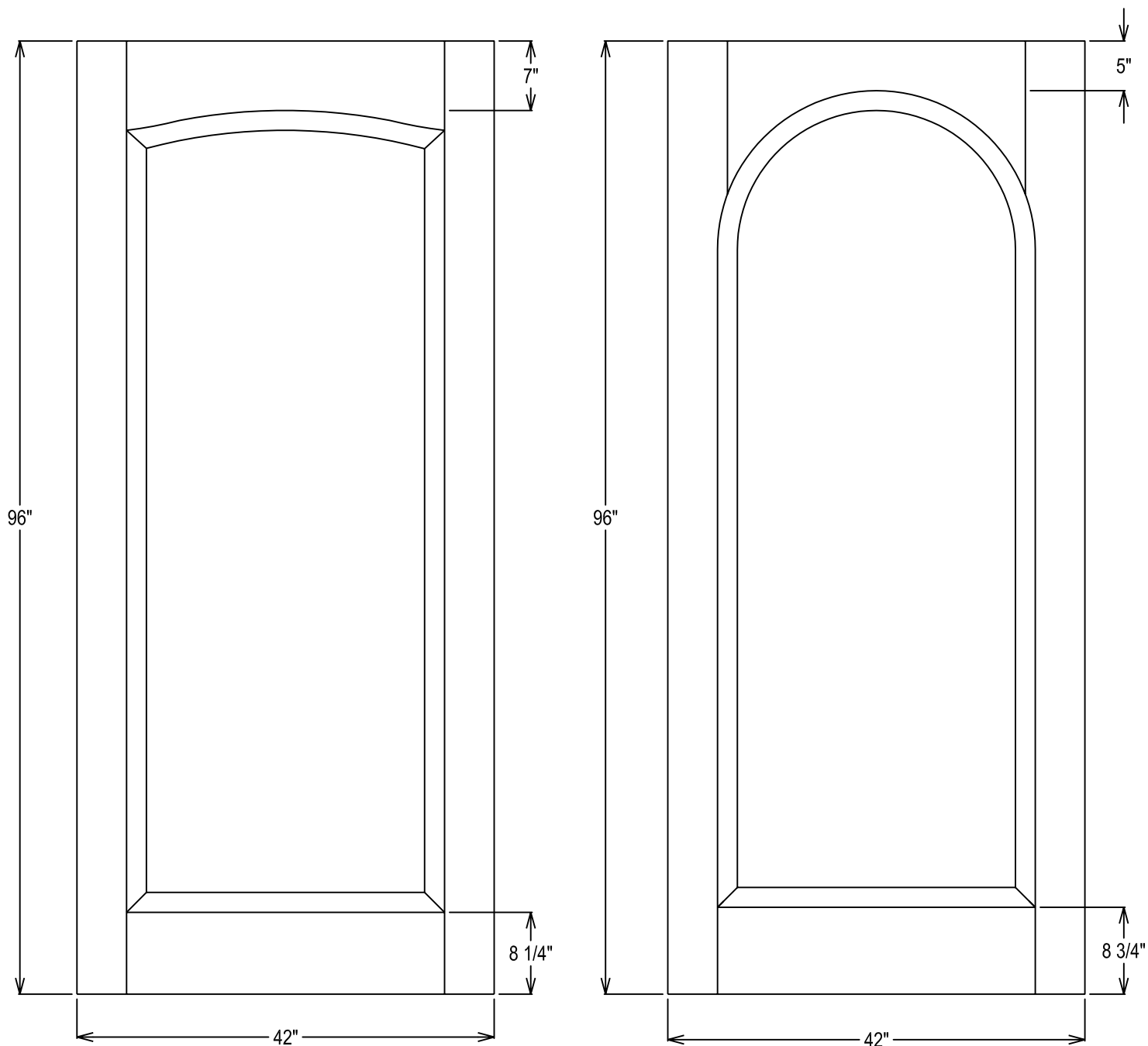
20-Minute Rating, 1-Panel Layout
