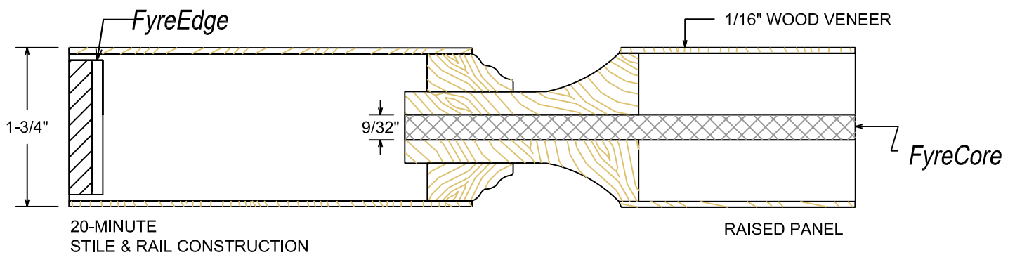
20-Minute Rating, 8&12-Panel Layout
