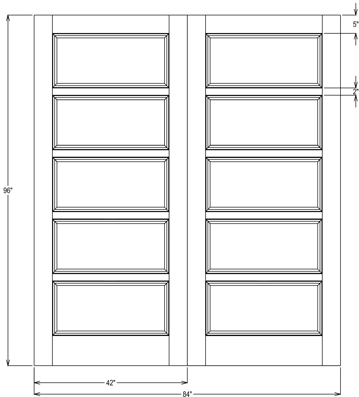
20-Minute Rating, Paired Doors, 5-Panel Layout
