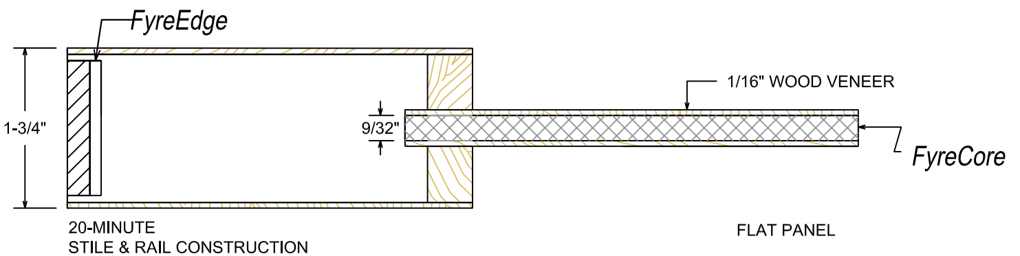
20-Minute Rating, 1-Panel Layout
