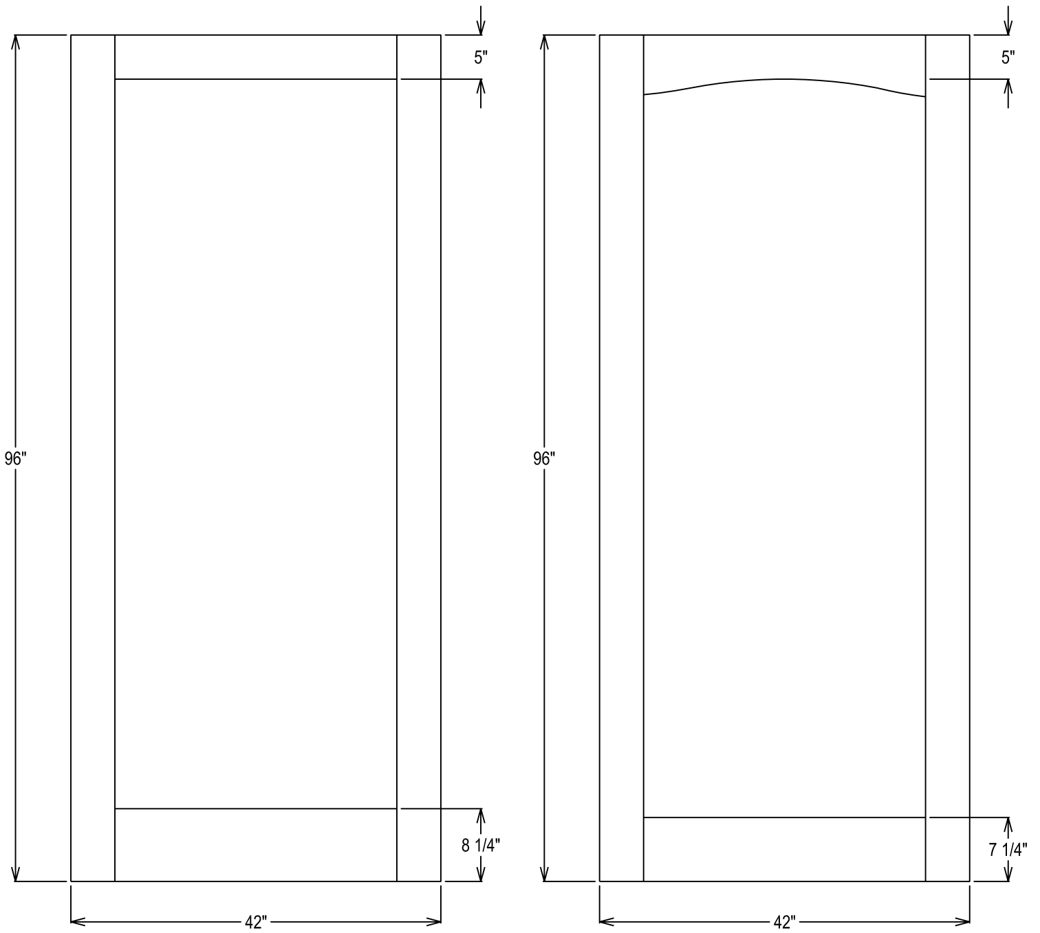
20-Minute Rating, 1-Panel Layout
