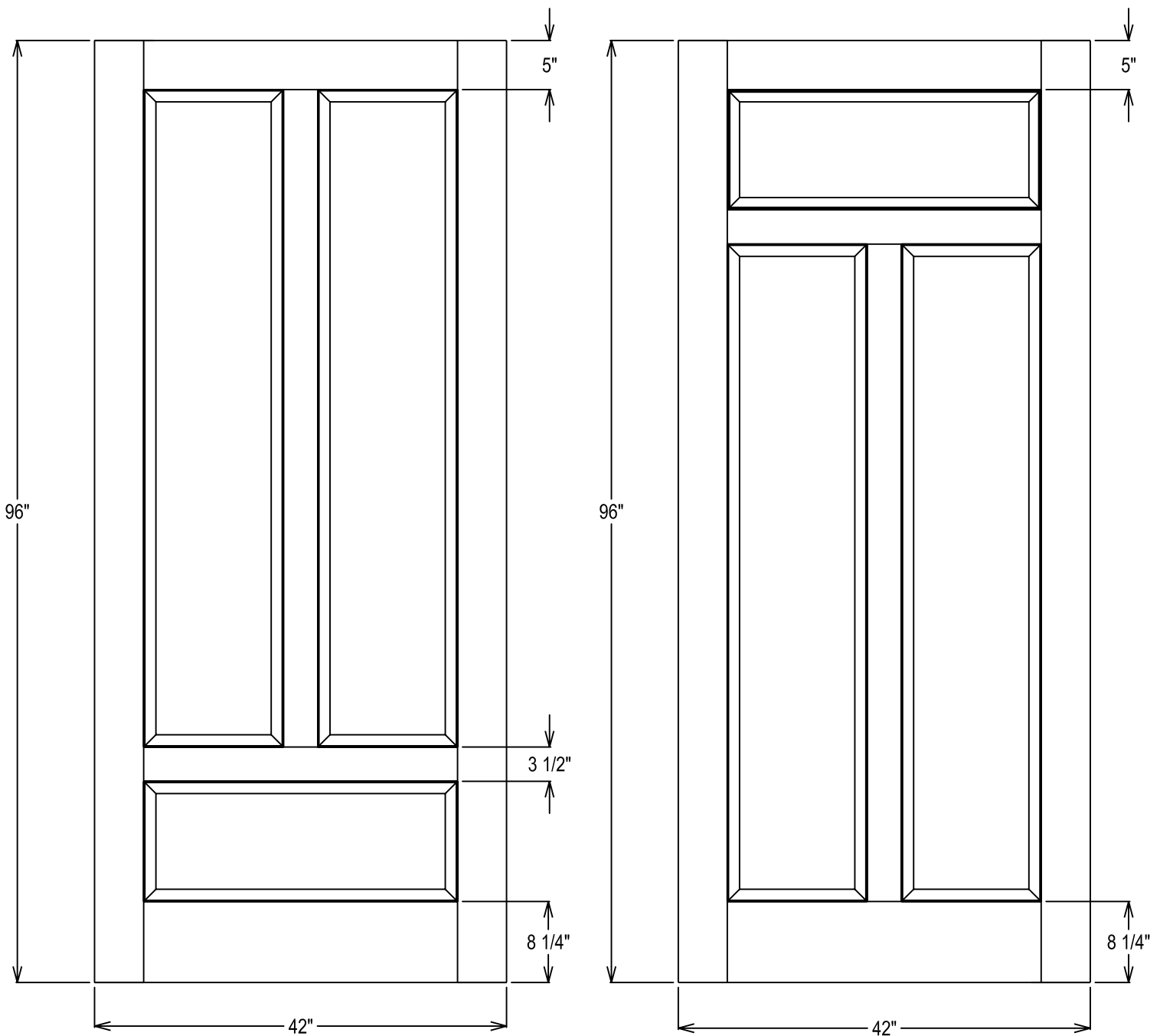
20-Minute Rating, 3-Panel Layout
