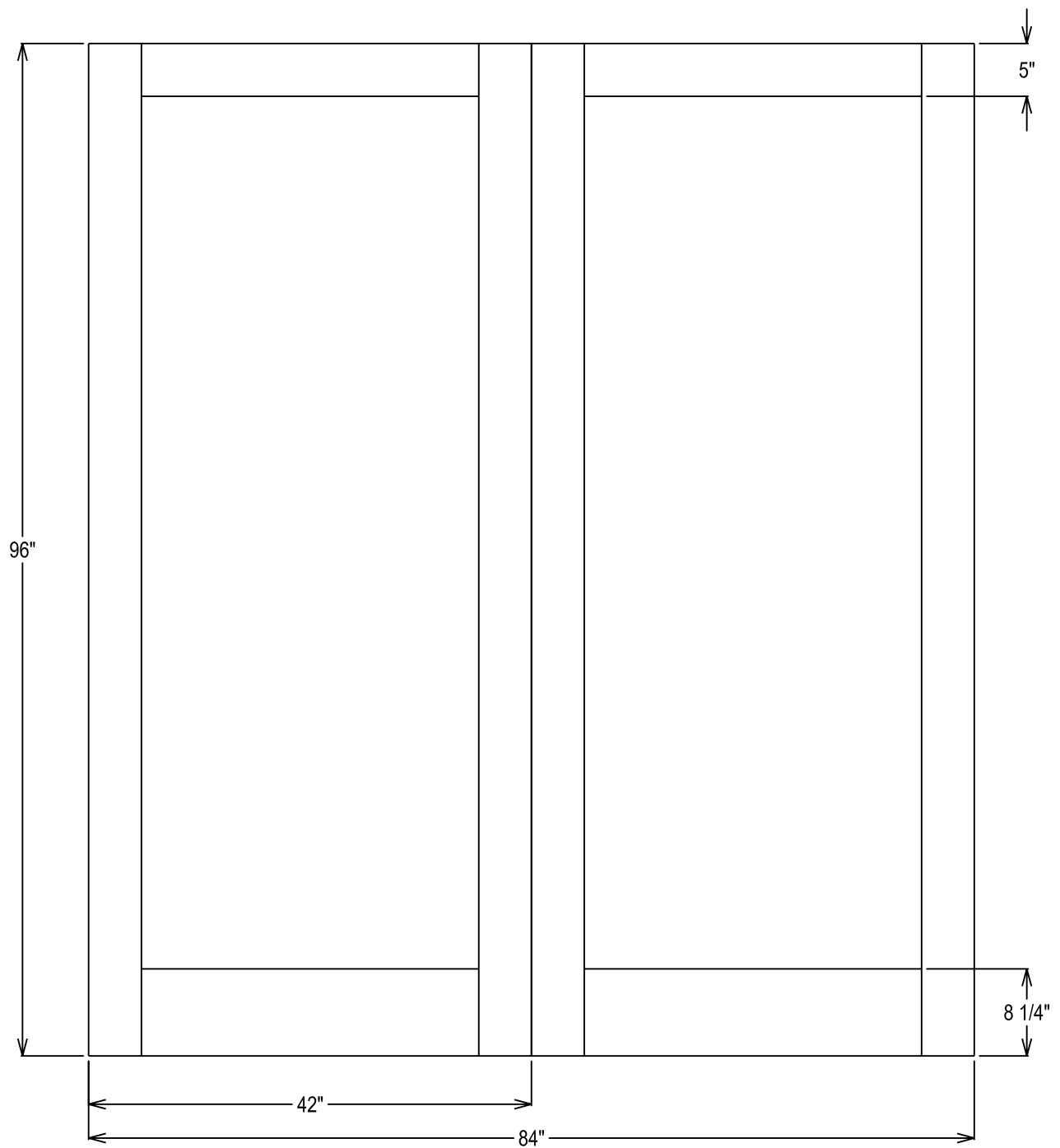
20-Minute Rating, Paired Doors, 1-Panel Layout
