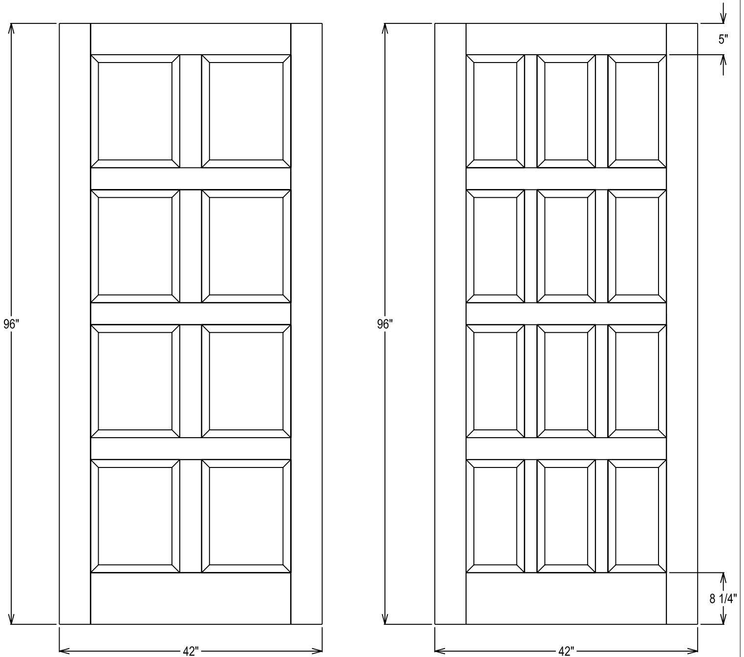
20-Minute Rating, 8&12-Panel Layout
