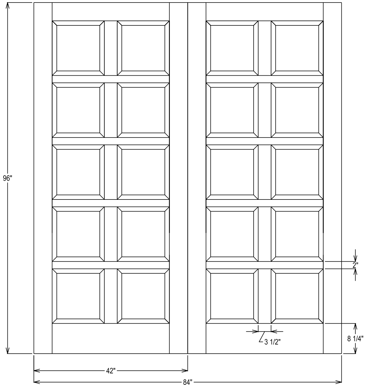
20-Minute Rating, Paired Doors, 10-Panel Layout
