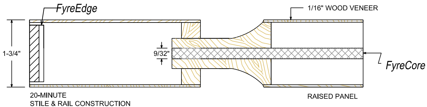
20-Minute Rating, 1-Panel Layout
