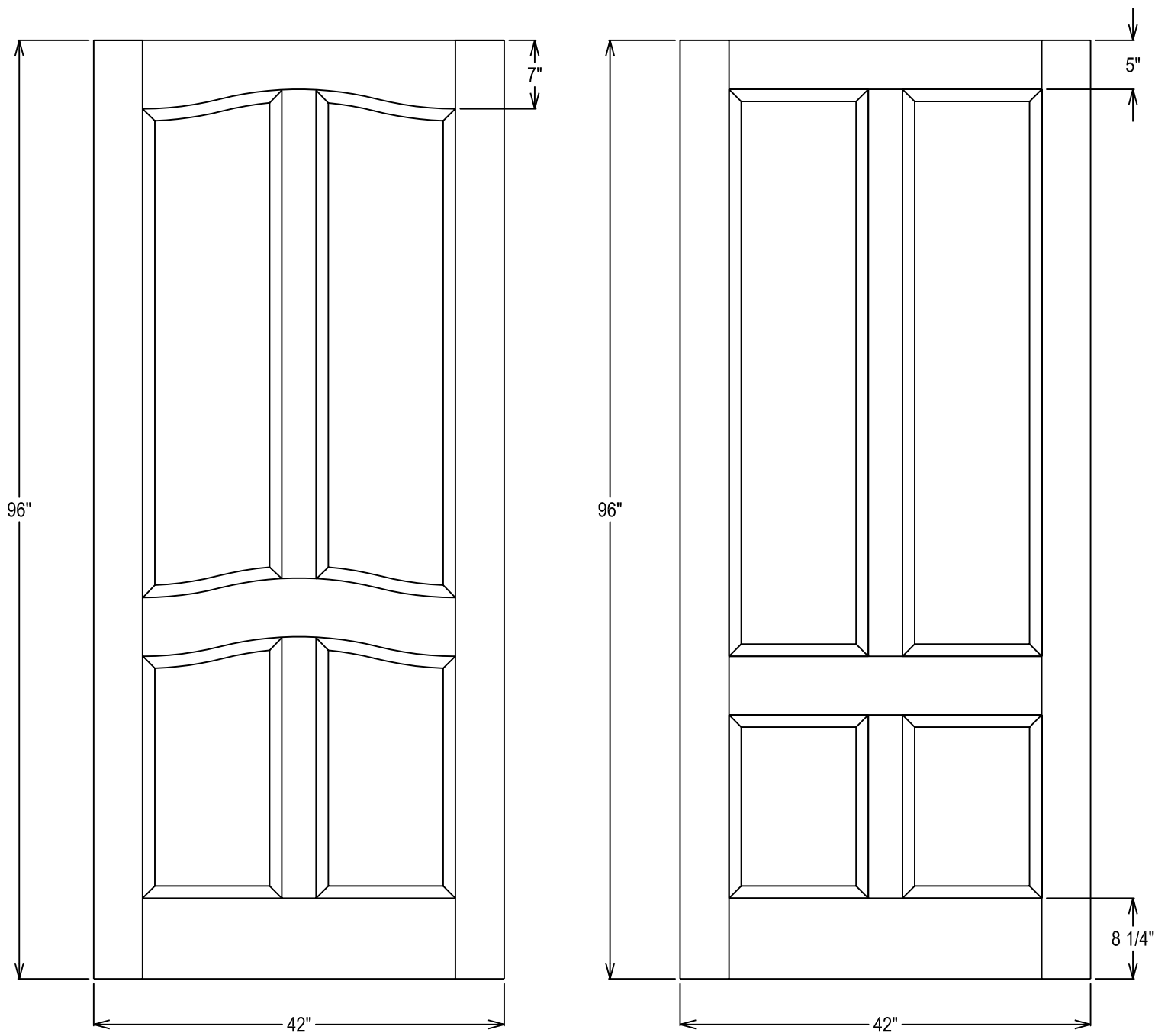
20-Minute Rating, 4-Panel Layout
