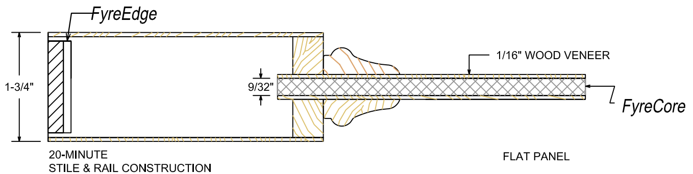
20-Minute Rating, Paired Doors, 2-Panel Layout
